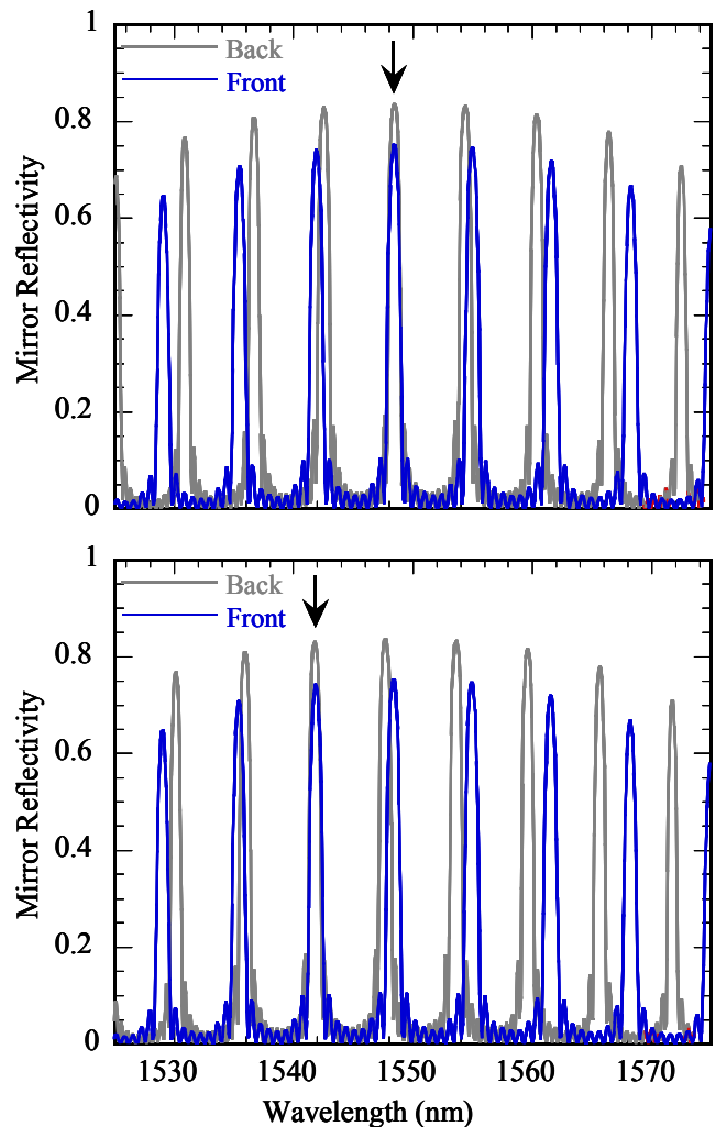
Figure 2: Overlaid mirror reflectivity spectra calculated for two different back mirror current levels. A small change in back mirror index results in a large shift in lasing wavelength (Vernier effect).
