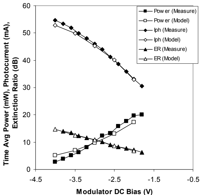
Figure 12: Device output power, photocurrent, and extinction ratio under RF operation: measured values (solid symbols) and model (open symbols). The DC bias is varied and the peak-to-peak RF driver bias is 3.4 V, with a modulation rate of 2.5 Gb/s. Operating wavelength is 1545 nm.
