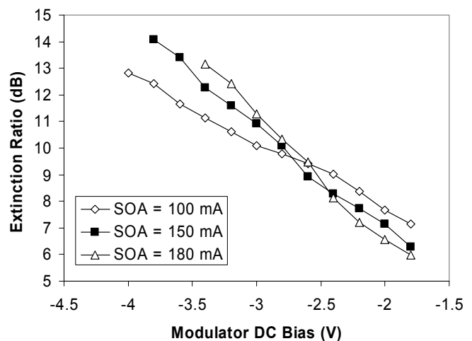
Figure 11: Measured RF extinction ratio as a function of modulator DC bias. The RF driver voltage is kept constant at 3.4V peak-to-peak, and modulation rate is 2.5 Gb/sec. Operating wavelength is 1545 nm. SOA current is varied.
