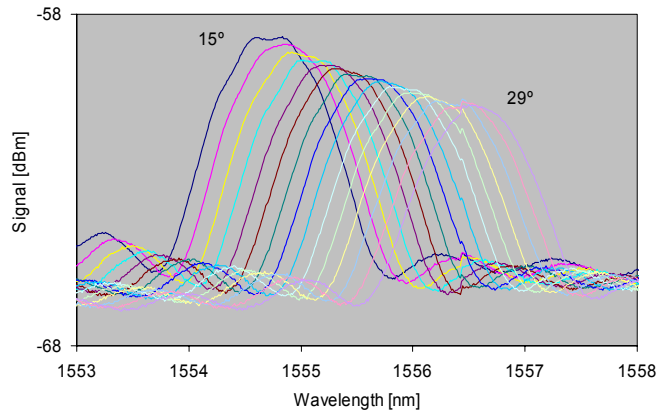
Figure 4: Front mirror peaks observed by driving the amplifier section at a fixed current and varying the stage temperature from 15°C to 29°C in increments of 1°C.
