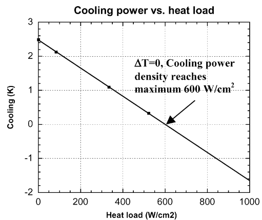
Fig. 4. Maximum cooling temperature versus heat load for a typical SiGe microrefrigerator (size: 40 \times 40 \mu\text{m}^2 ). By definition, at maximum cooling power density, cooling temperature is zero. Since there is a linear relationship, if heat load power density is, e.g., a factor of two smaller than the maximum value ( 300 \text{ W/cm}^2 ), cooling by a factor of two smaller than the maximum value ( 1.2 \text{ C} ) can be achieved at the same time.
