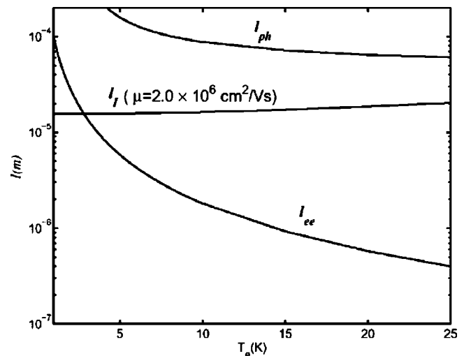
FIG. 3. The electron–impurity ( l_I ), electron–phonon ( l_{ph} ), and electron–electron scattering lengths for a 2DEG with the mobility \mu(T=0) = 2 \times 10^6 \text{ cm}^2/\text{Vs} and density n = 2.7 \times 10^{11}/\text{cm}^2 . The lattice temperature T_L is fixed at 1 K and the electron temperature T_e is varied.
